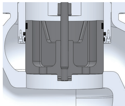
③ Balance plug: For high pressure, large valve size, with low thrust requested.
