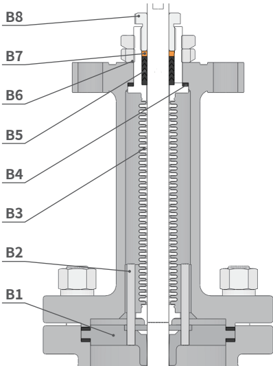
Metal Bellows Seal
